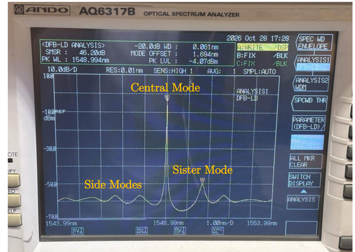
Optical Spectrum of a DFB Laser
